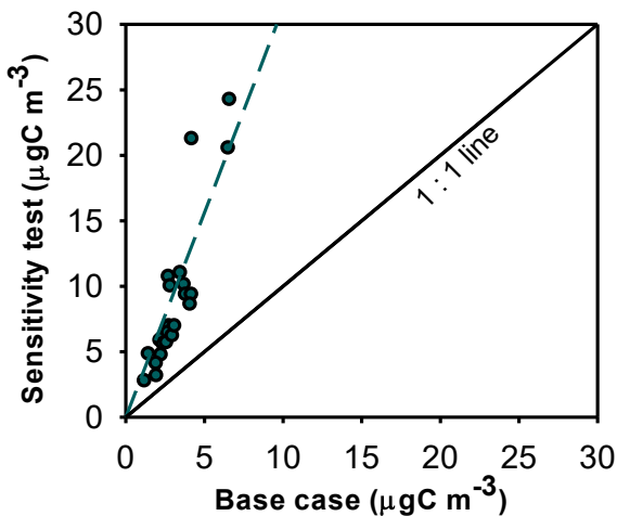
(a) Garbage burning contribution to OC
