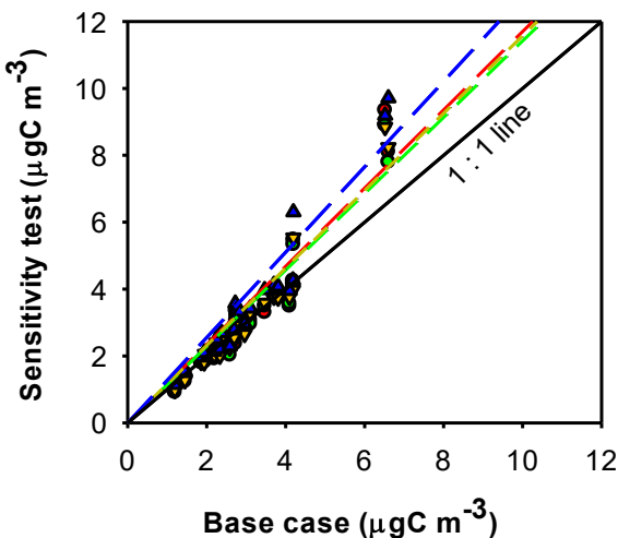
(b) Biomass burning contribution to OC
