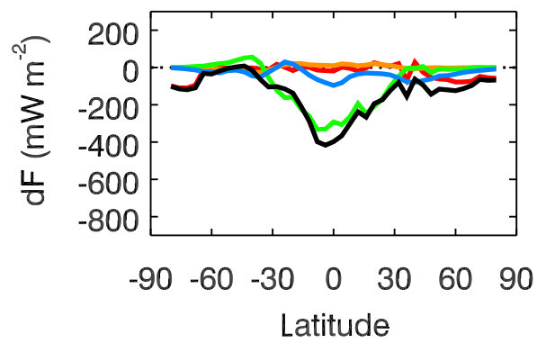
EMAC-L90MA
