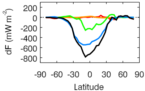
MRI-ESM1r1
