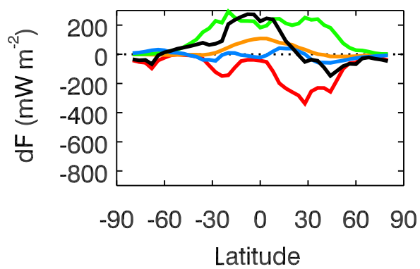
MRI-ESM1r1
