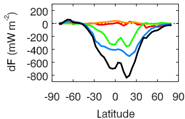
EMAC-L47MA
