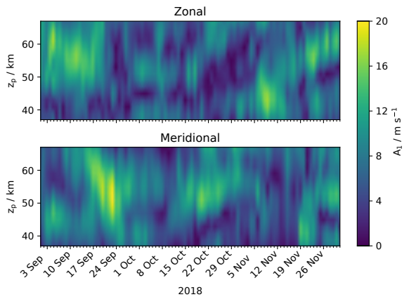
(c) MERRA-2 composite amplitude A_1
