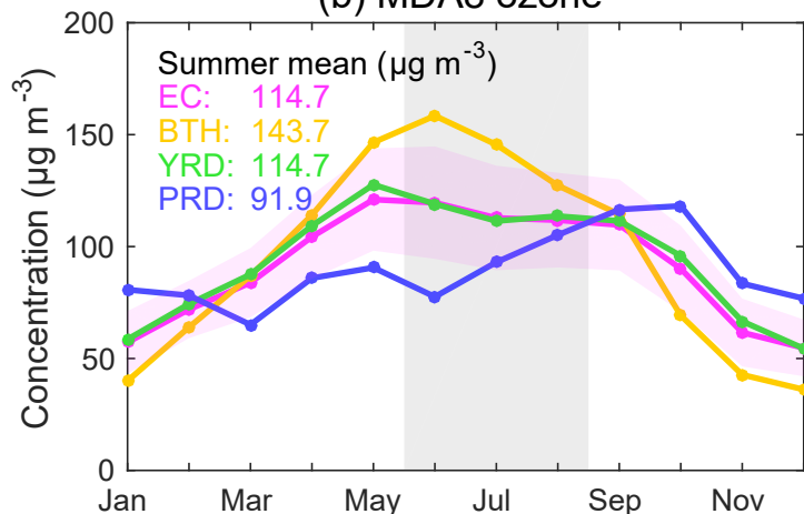
(b) MDA8 ozone
