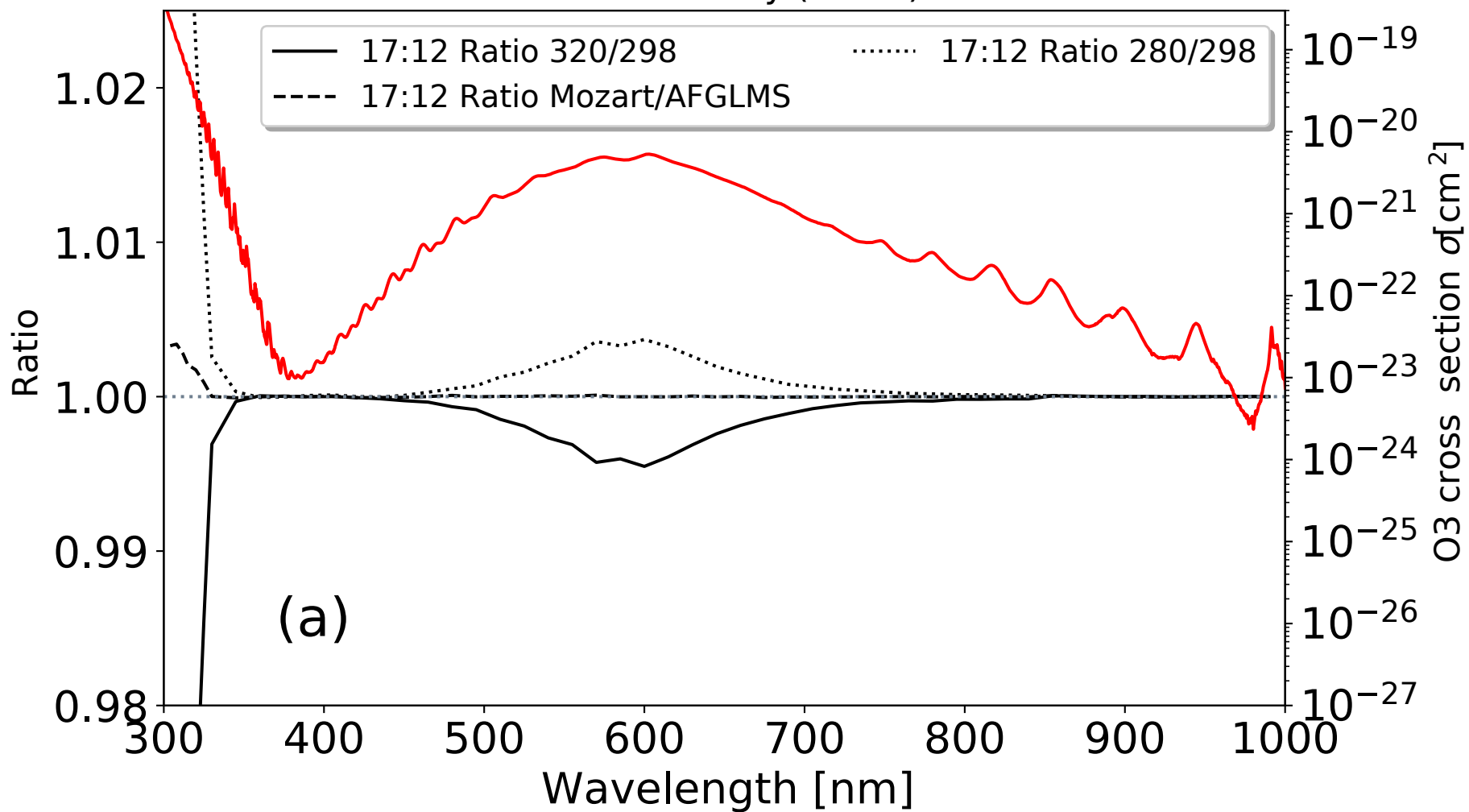
Outside totality (17:12)
