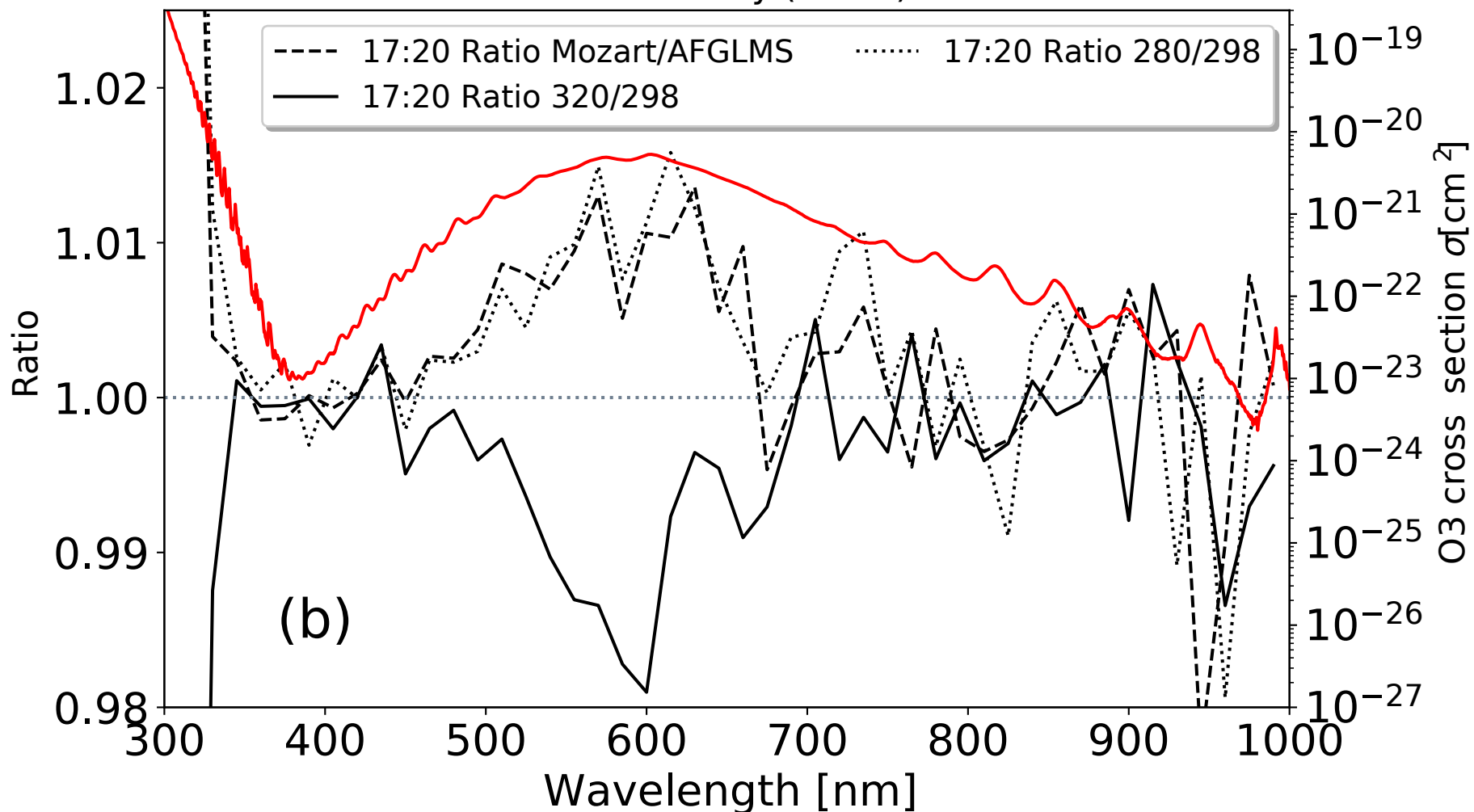
Inside totality (17:20)
