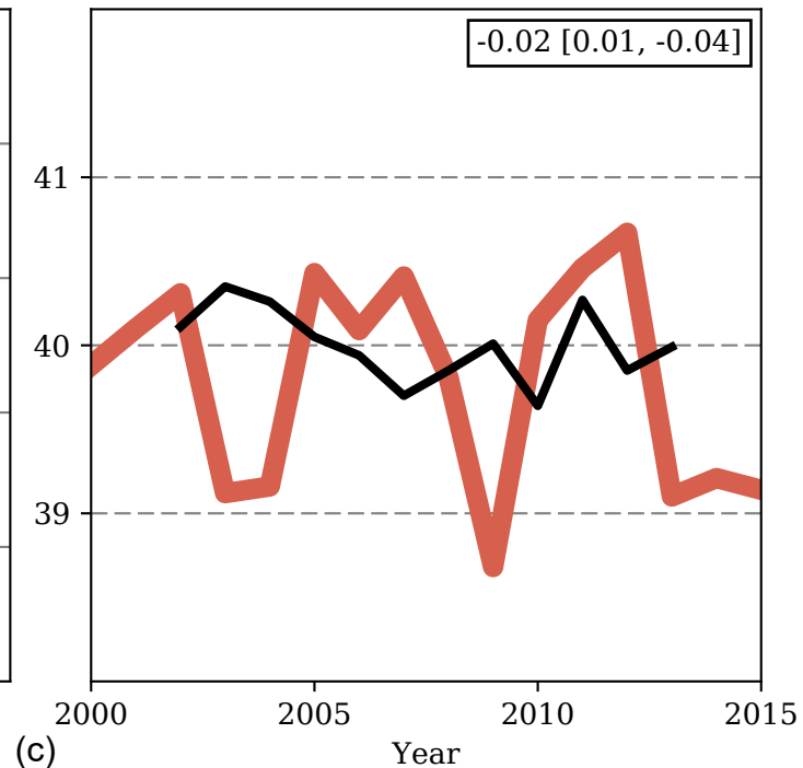
Pop. weighted MDA8 conc. [ppb]
