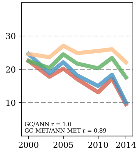
AOT40 soybeans [ppmh]
