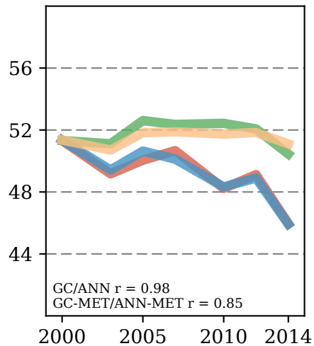
AOT40 wheat MJJ [ppmh]
