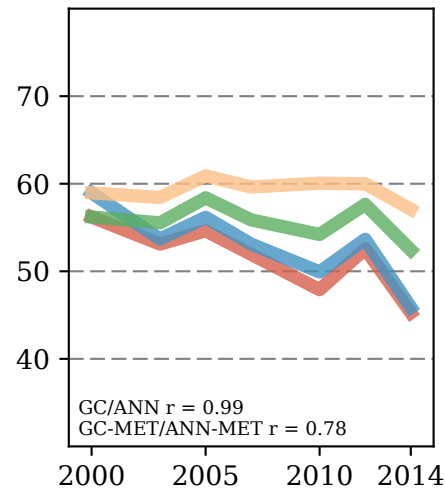
AOT40 maize [ppmh]
