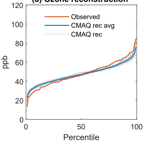
(a) Ozone reconstruction
