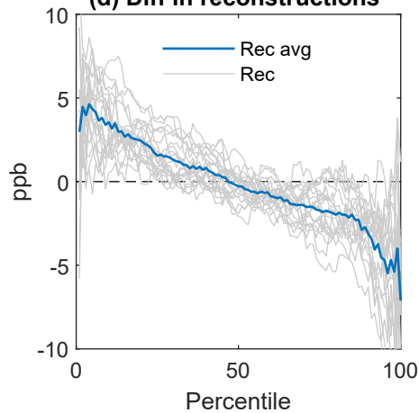
(d) Diff in reconstructions
