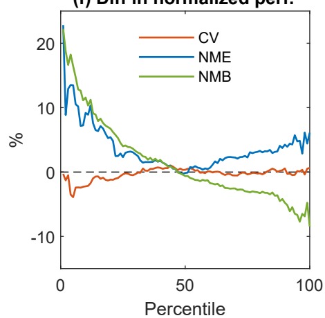
(f) Diff in normalized perf.
