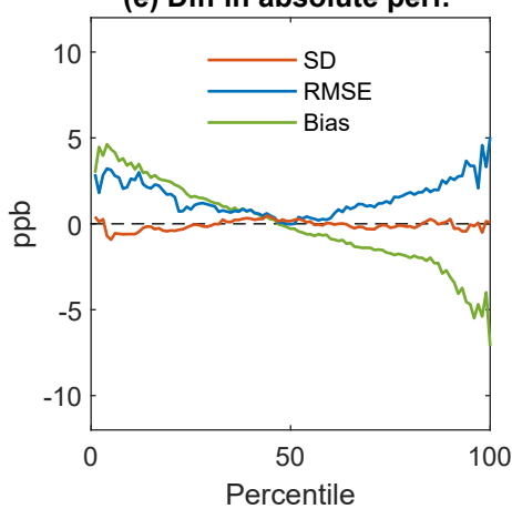
(e) Diff in absolute perf.
