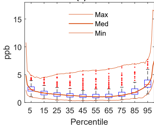
(a) SD
