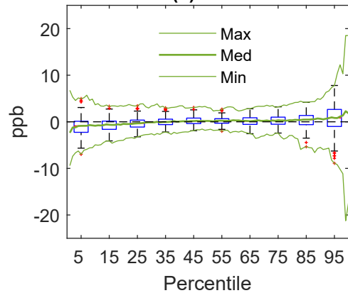
(c) Bias
