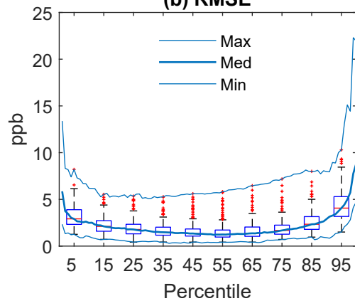
(b) RMSE
