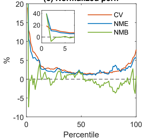
(c) Normalized perf.
