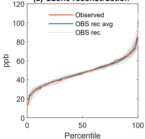
(a) Ozone reconstruction
