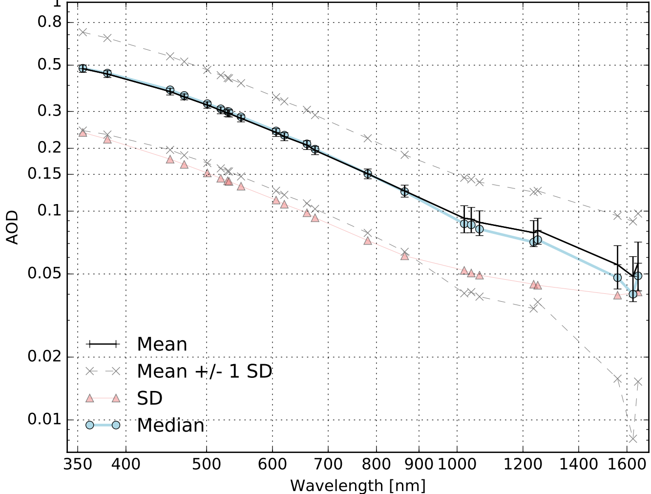
ACAOD average spectra from 4STAR at selected wavelengths
