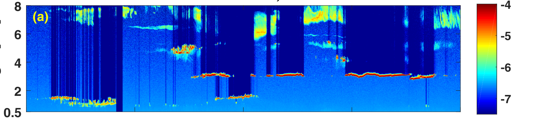
Volume depolarization ratio, 22 March 2019
