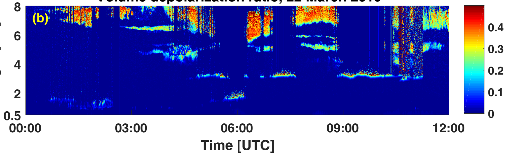
Volume depolarization ratio, 22 March 2019
