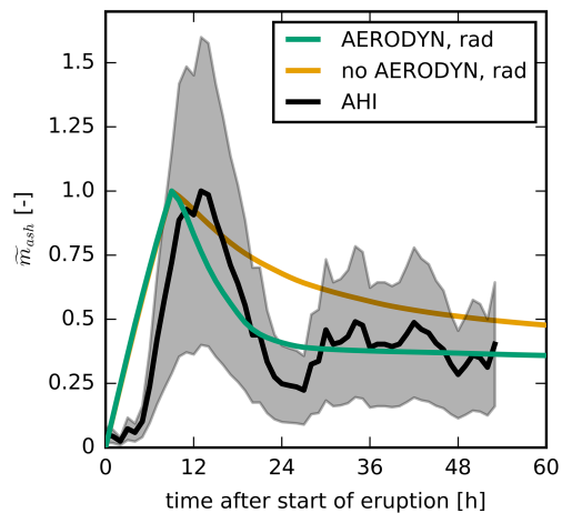
Figure 7. Normalized total volcanic ash mass \tilde{m}_{\text{ash}} over the time after the onset of the volcanic eruption on 21 June 2019 at 18:00 UTC. The green and yellow curves represent AERODYN-rad and no_AERODYN-rad, respectively. The black curve is based on AHI measurements with an error estimate in gray.
