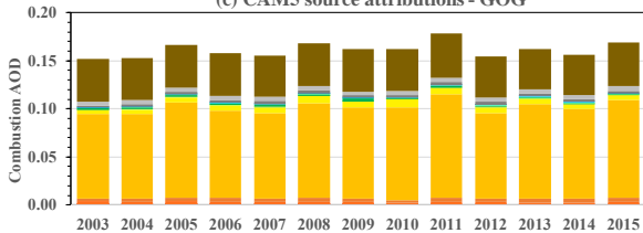
(c) CAM5 source attributions - GOG
