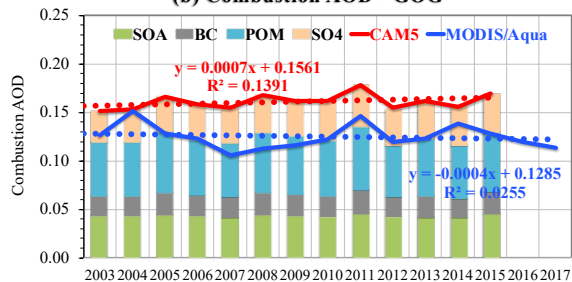
(b) Combustion AOD - GOG
