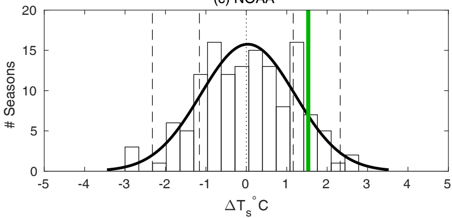
(c) NOAA
