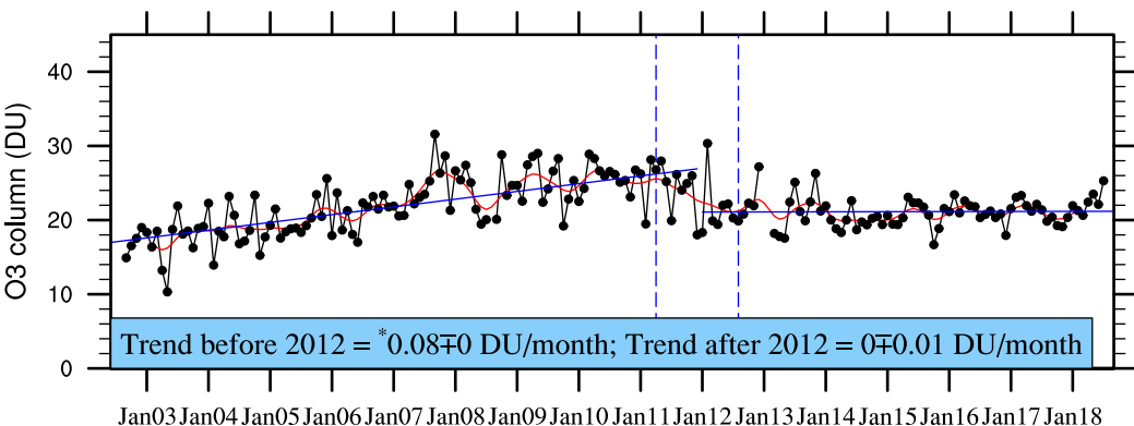
(b) Deseasonalized 3 - 9 km O 3 column by ozonesonde
