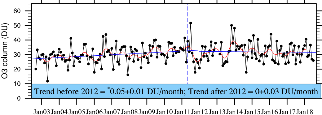
(b) Deseasonalized 3 - 9 km O 3 column by ozonesonde
