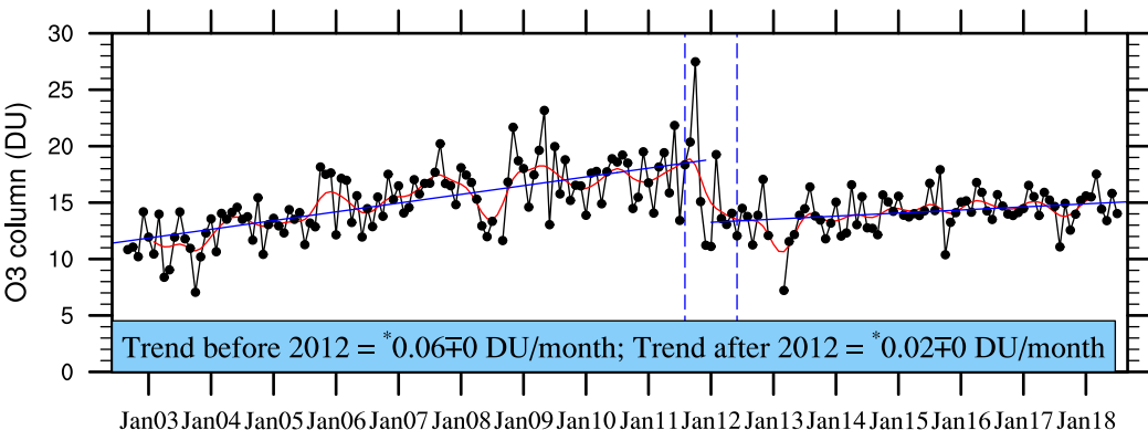
(c) Deseasonalized 0 - 3 km O 3 column by ozonesonde
