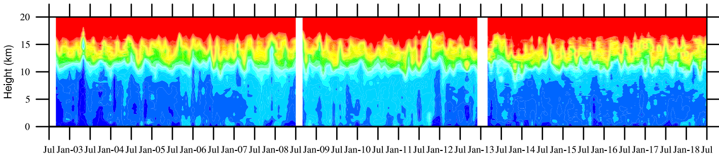
(a) Deseasonalized ozone mixing ratio by IAP ozonesondes
