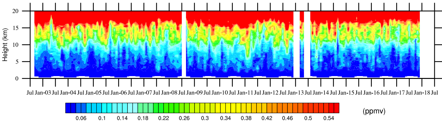
(b) Deseasonalized ozone mixing ratio by CLaMS
