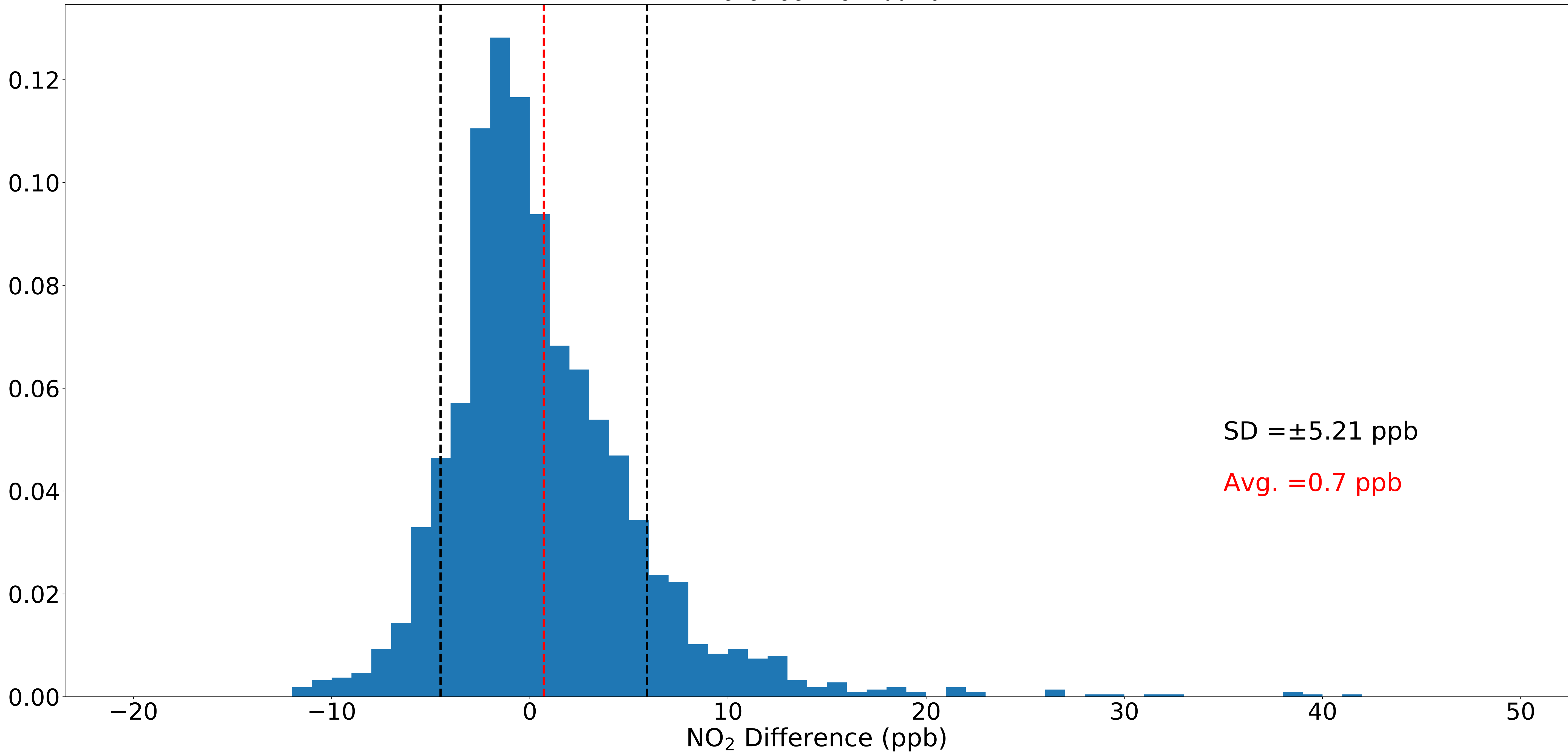
Difference Distribution
