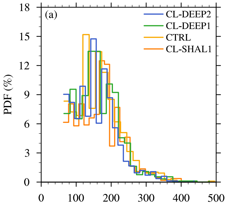
Cloud-layer depth
