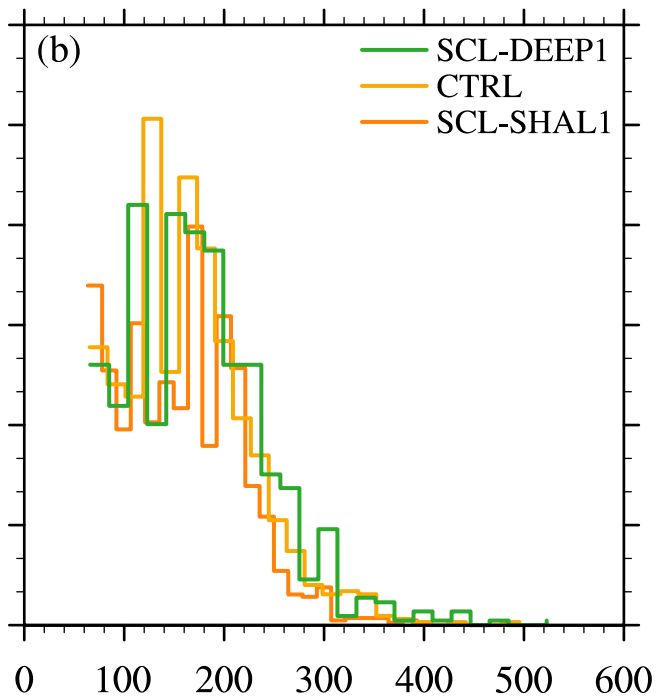
Subcloud-layer depth
