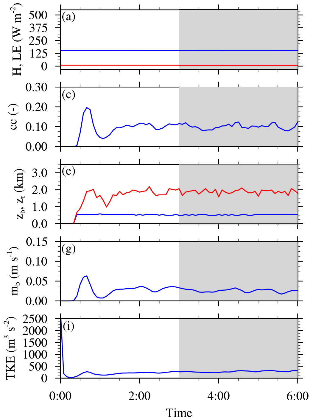
BOMEX
