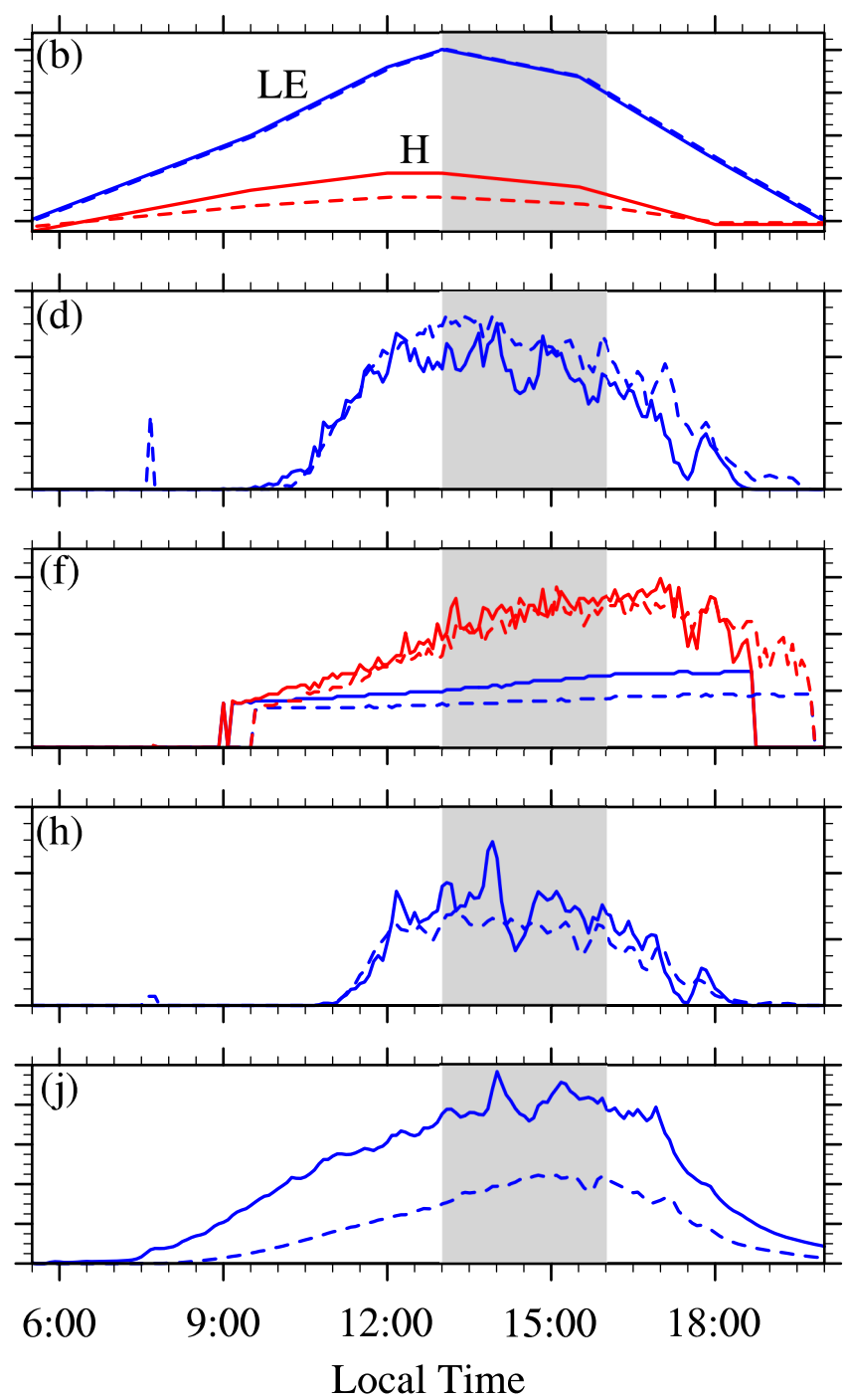
ARM-SGP
