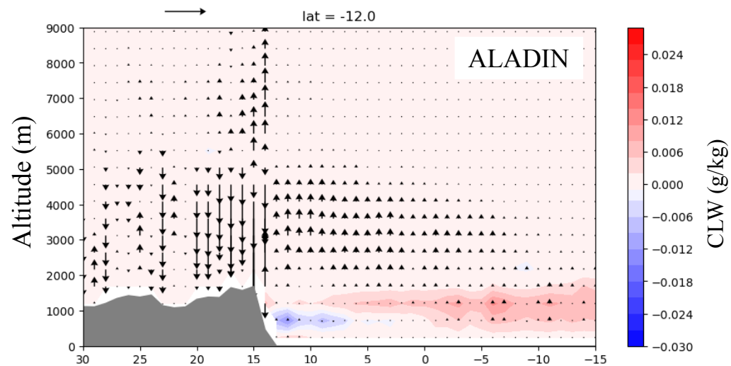
(b) Vertical Velocity / Liquid water - 12S / JAS 2000-2015
