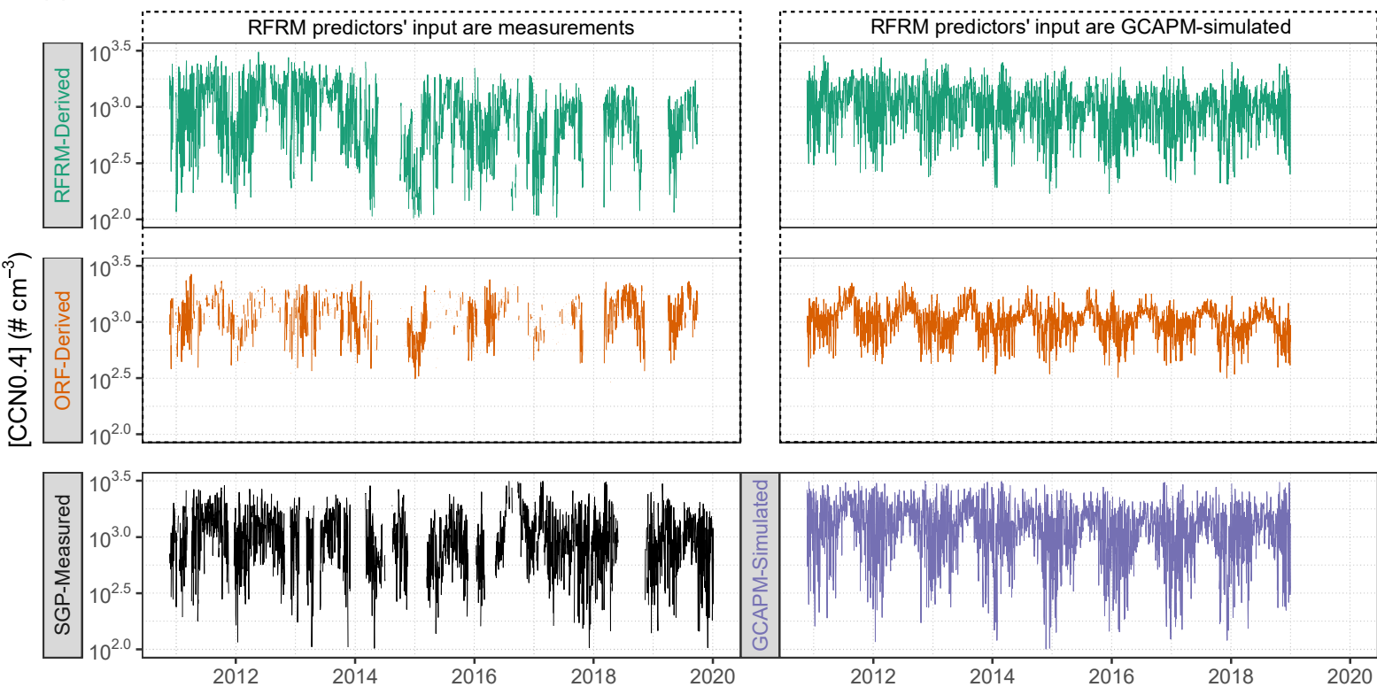
(a) [CCN0.4] time series for the SGP site
