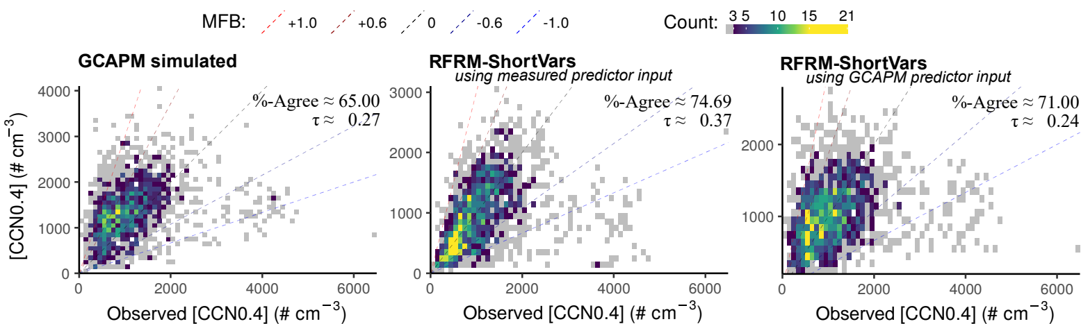
(b) Performance comparison of GCAPM and RFRM [CCN0.4] versus measurements for the SGP site
