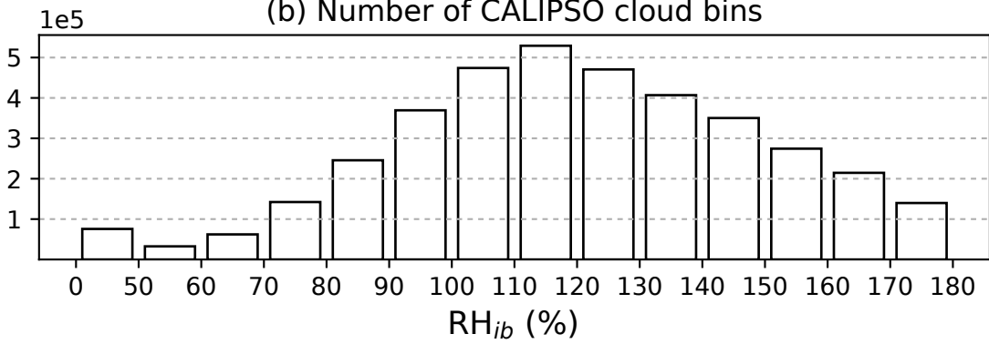
(b) Number of CALIPSO cloud bins
