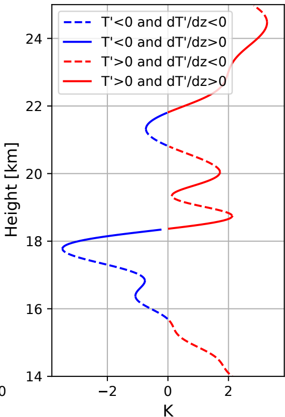
(b) Temperature anomaly and its phases
