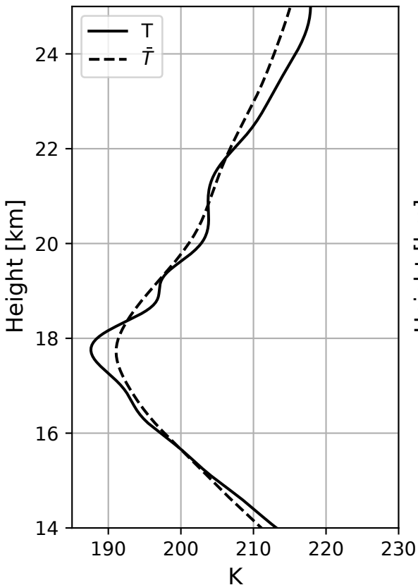
(a) Temperature and corresponding mean state
