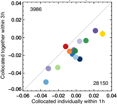
Biases (world)
