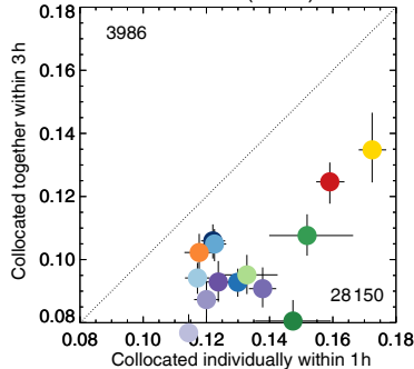
RMSDs (world)
