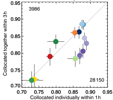
Correlations (world)
