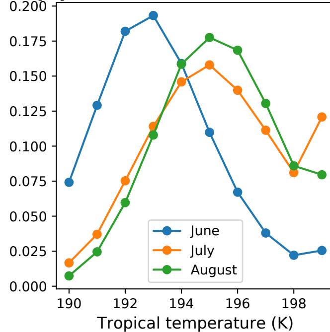
(b) Tropical temperature
