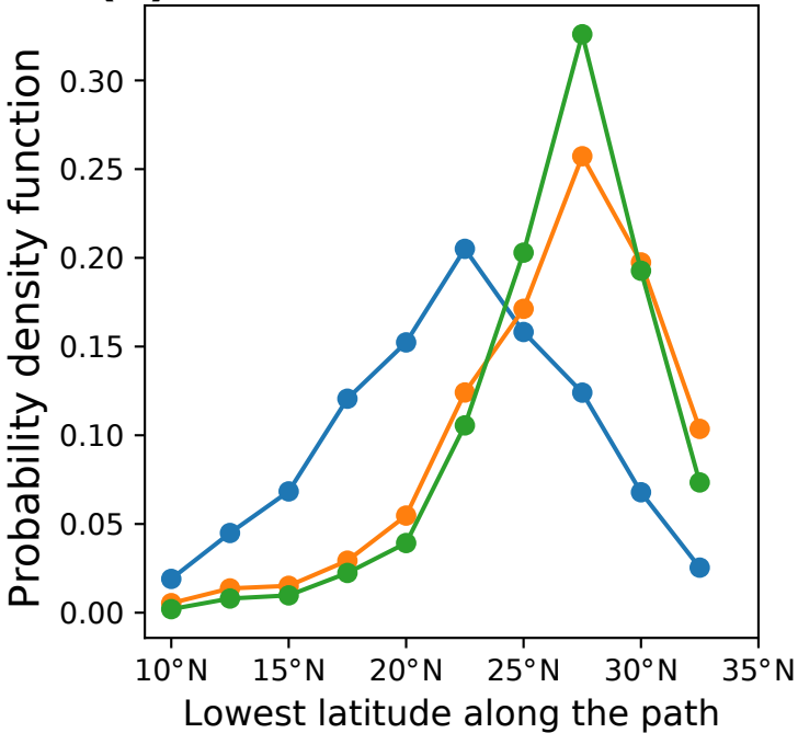
(a) Lowest latitude along the path
