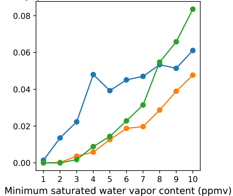
(c) Minimum saturated water vapor
