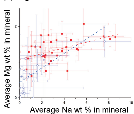
(c) Mg vs. Na
