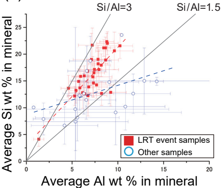
(a) Si vs. Al
