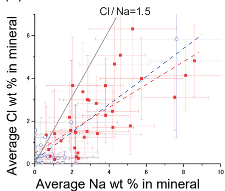
(b) Cl vs. Na
