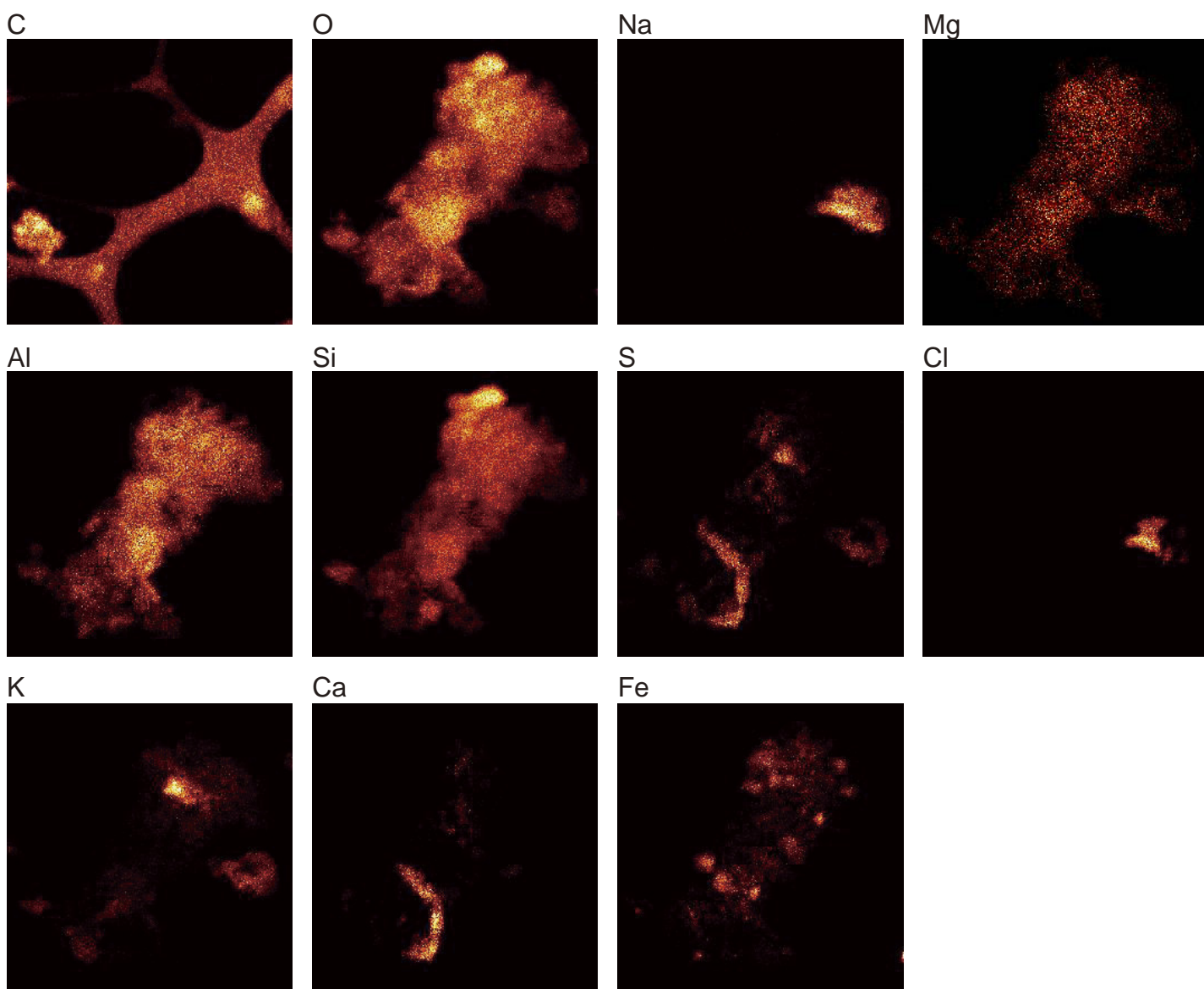
(c) Element mapping images
