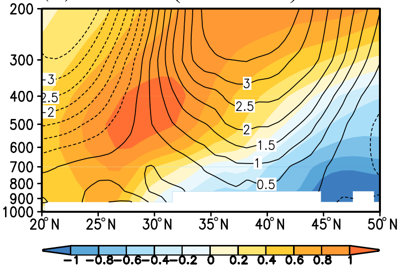
(a) T & U (76–110° E)
