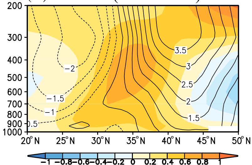
(b) T & U (140–162° E)
