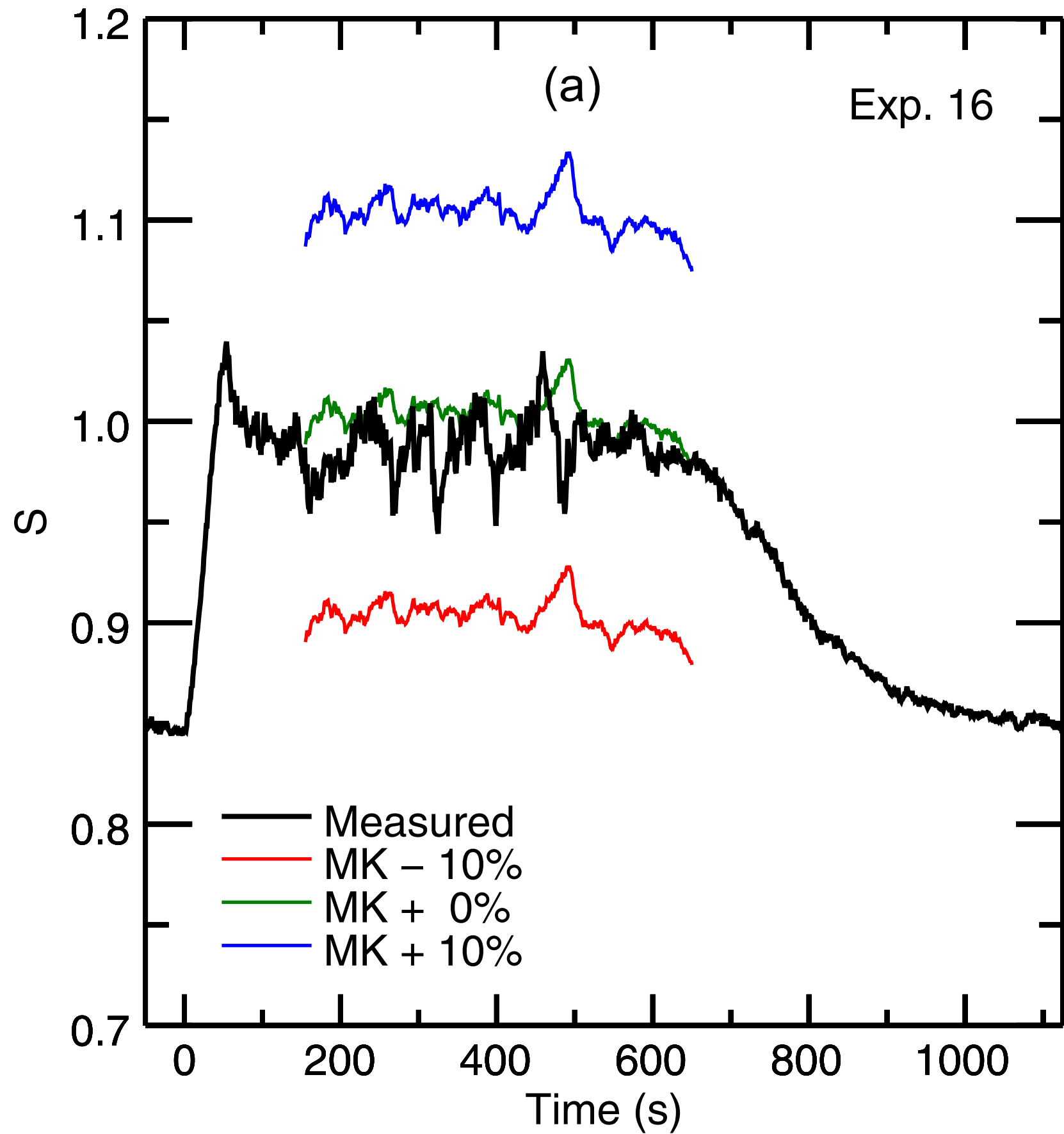
Cirrus dominated
