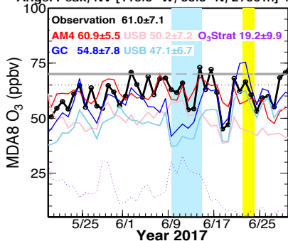
Angel Peak, NV [115.6° W, 36.3° N, 2700 m] Mesa Verde NP, CO [108.5° W, 37.2° N, 2165 m] Joe Neal, NV [115.2° W, 36.3° N, 709 m]
