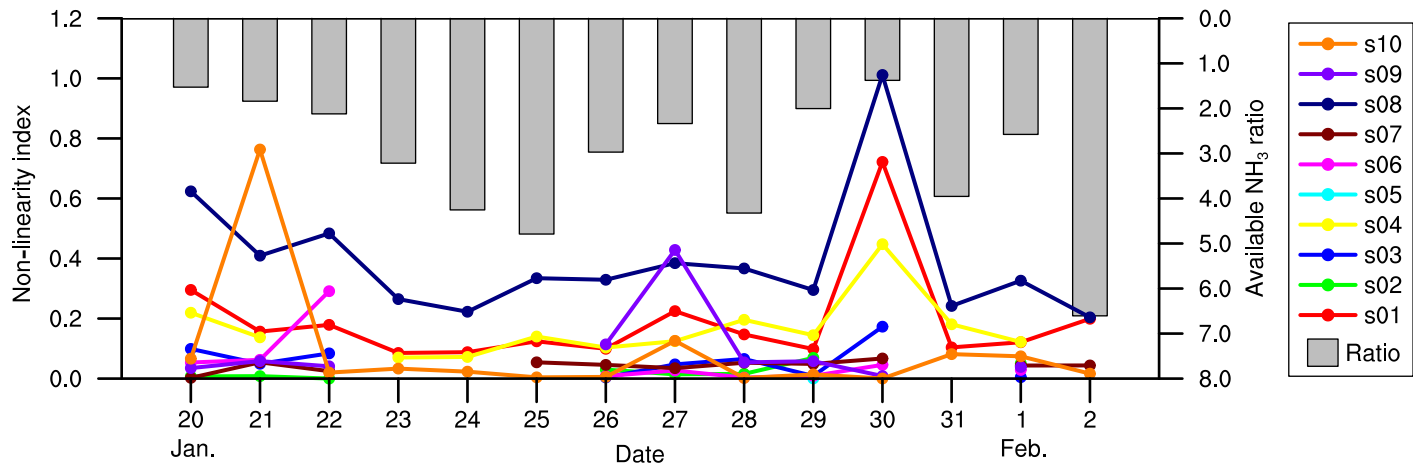
(b) Non-linearity index and available \text{NH}_3 ratio
