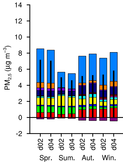
(b3) PM 2.5 (ST)
