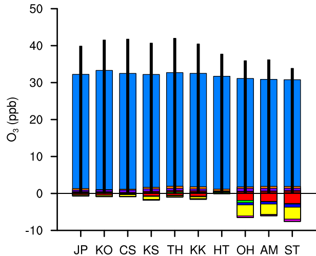
(a) O 3
