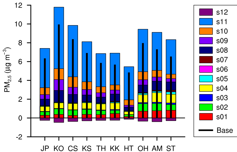
(b) PM 2.5
