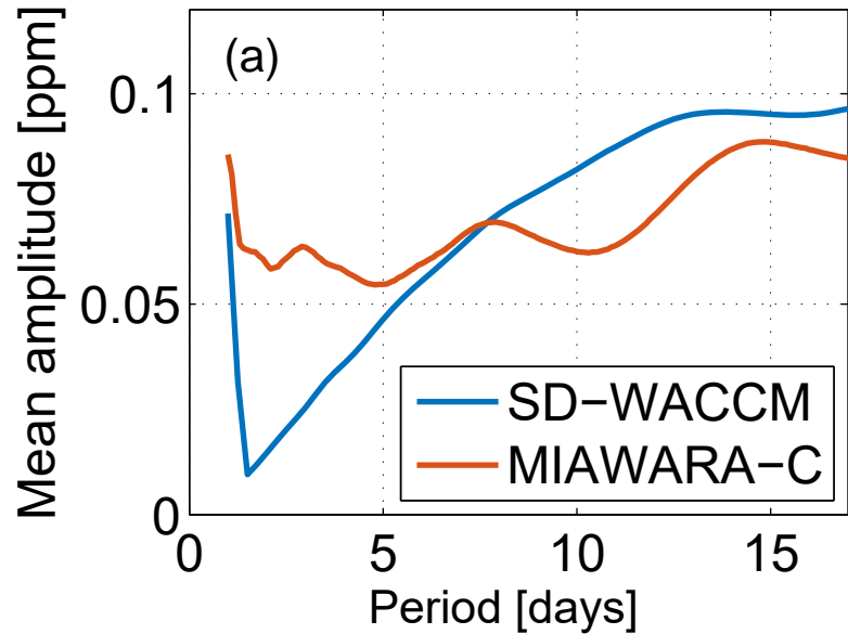
O 3 : 5–50 hPa, summer
