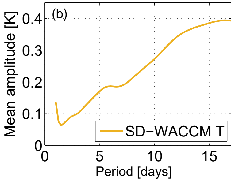
T: 5–50 hPa, summer
