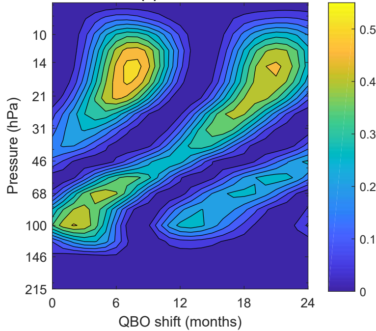
(b) QBO R^2
