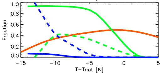
WACCM_ccmi
