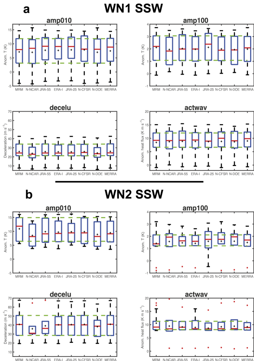
5 Figure S1. Box plots showing the distribution of the dynamical benchmarks of (a) WN1 SSWs and (b) WN2 SSWs in the comparison periods. The interquartile range is represented by the size of the box and the red line (black cross) corresponds to the median (mean). Whiskers indicate the maximum and minimum points in the distribution that are not outliers. Outliers (red crosses) are defined as points with values greater than 3/2 times the interquartile range from the ends of the box.
