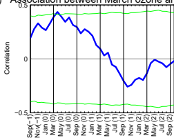
(j) Association between March ozone and ENSO
