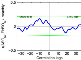
(i) NIWA-R3-2052-2092
