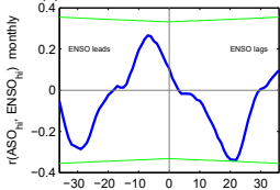
(a) ASO vs. ENSO MERRA/SWOOSH
