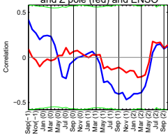
(b) Association between March ozone (blue) and Z pole (red) and ENSO
