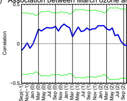
(h) Association between March ozone and ENSO
