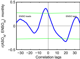
(c) WACCM-R3-2011-2051
