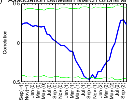
(d) Association between March ozone and ENSO
