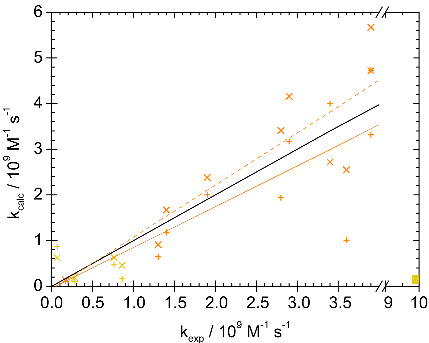
(c) Carbonyl compounds
