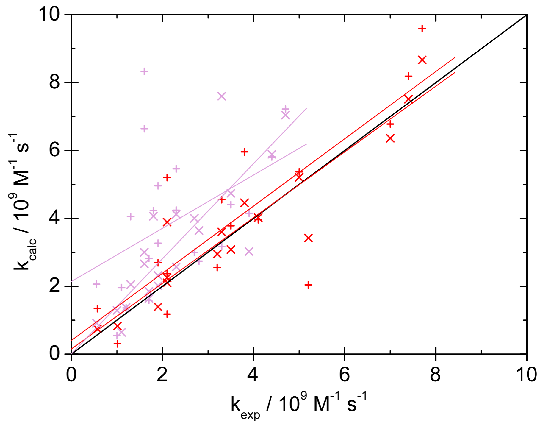
(b) Alcohol compounds
