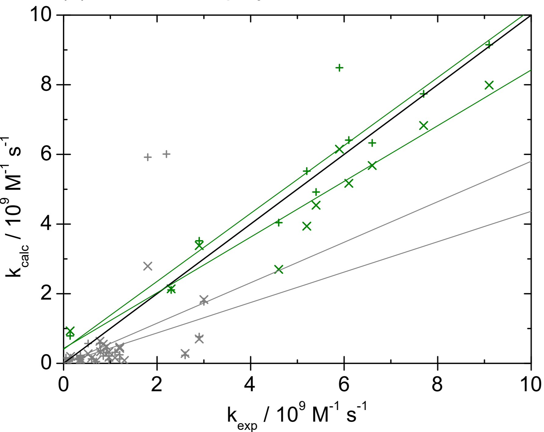
(a) Alkanes and polyfunctionals
