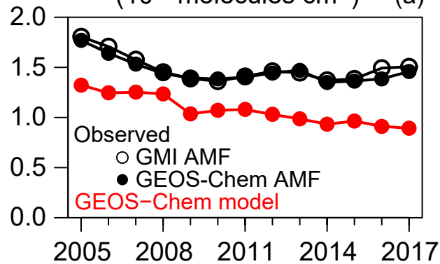
NO 2 vertical column density (10 15 molecules cm -2 ) (a)
