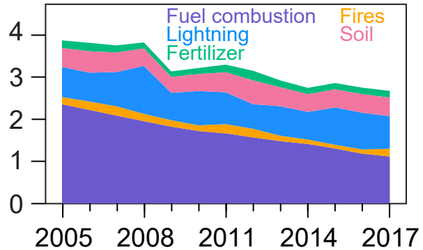
GEOS-Chem NO x emissions (Tg N a -1 ) (c)
