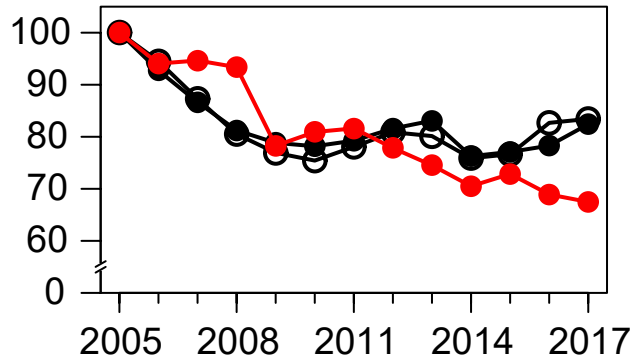
Change relative to 2005 (%) (b)
