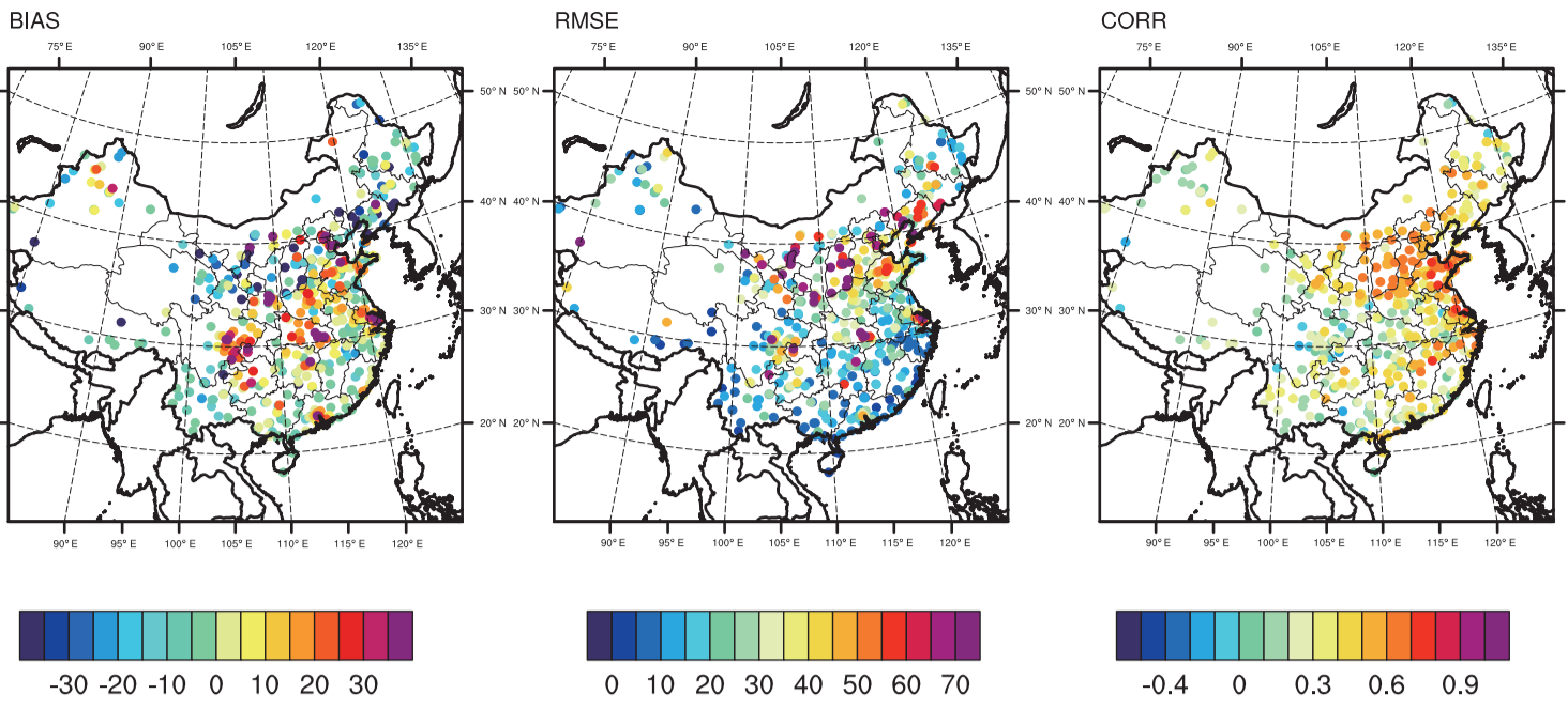
Differences (EMIS_DA_FCST - NO_DA_FCST) (b) Group A
