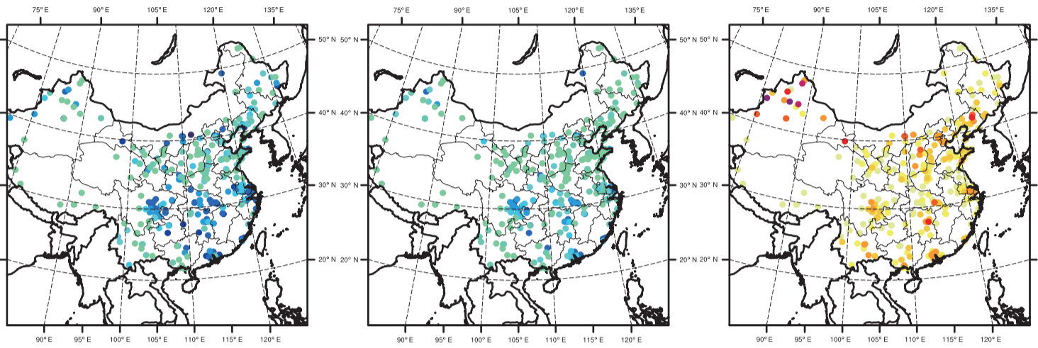
Differences (EMIS_DA_FCST - NO_DA_FCST) (b) Group A
