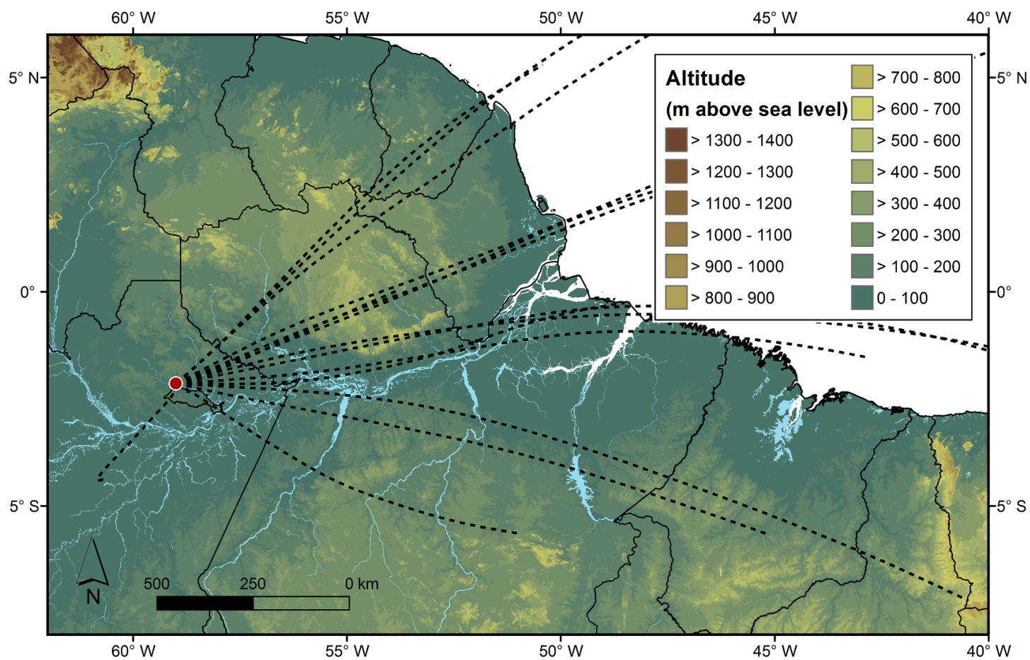
Figure S13. Map of the ATTO-relevant eastern Amazon Basin ( \text{ROI}_{\text{foot}} ) combining the backward trajectory (BT) data with altitude data obtained from SRTM digital elevation model. The trajectory data is represented as center lines of the 15 BT clusters (black dashed lines, see Fig. 4).
