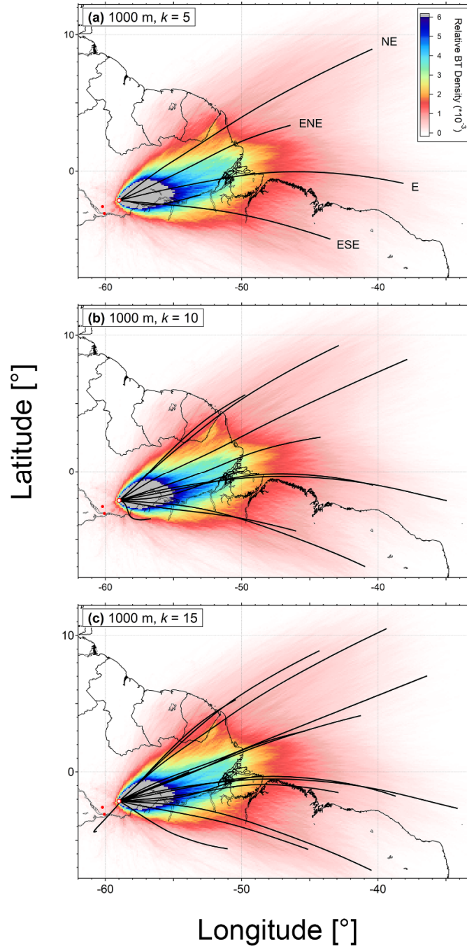
Figure S3. Air mass residence time maps, based on the entire ensembles of 3-day BTs (starting height 1000 m AGL, 01 Jan 2008 - 30 Jun 2016) with results from three k -means CA runs for k=5 , k=10 , and k=15 (compare Fig. S2).
