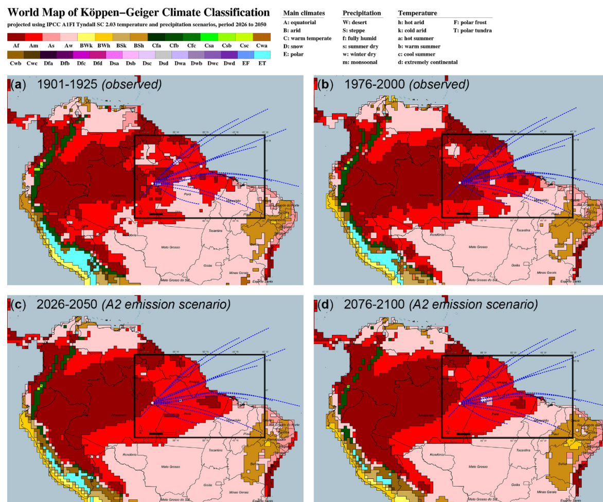
Figure S14. Map of the ATTO-relevant eastern Amazon Basin ( \text{ROI}_{\text{foot}} ) combining the backward trajectory (BT) data with the Köppen–Geiger climate classification for two observed periods ( a and b ), and projected based on the IPCC A2 emission scenario ( c and d ). The BT data is represented as center lines of the 15 BT clusters (blue dashed lines, see Fig. 4).
