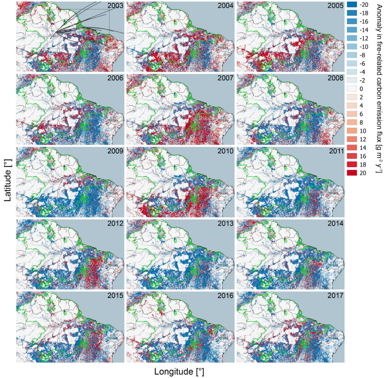
Figure S19. Anomalies in fire-related carbon emission based on GFAS-data for the ATTO-relevant eastern Amazon Basin (ROI foot ). Reference time period for anomalies is average from 2003 to 2017. For the year 2003, the BT data is represented as center lines of the 15 BT cluster (black dashed lines, exemplary for year 2003, see Fig. 4). The green line represents the boundaries of the biome of moist broadleaf forests according to Fig. 9.
