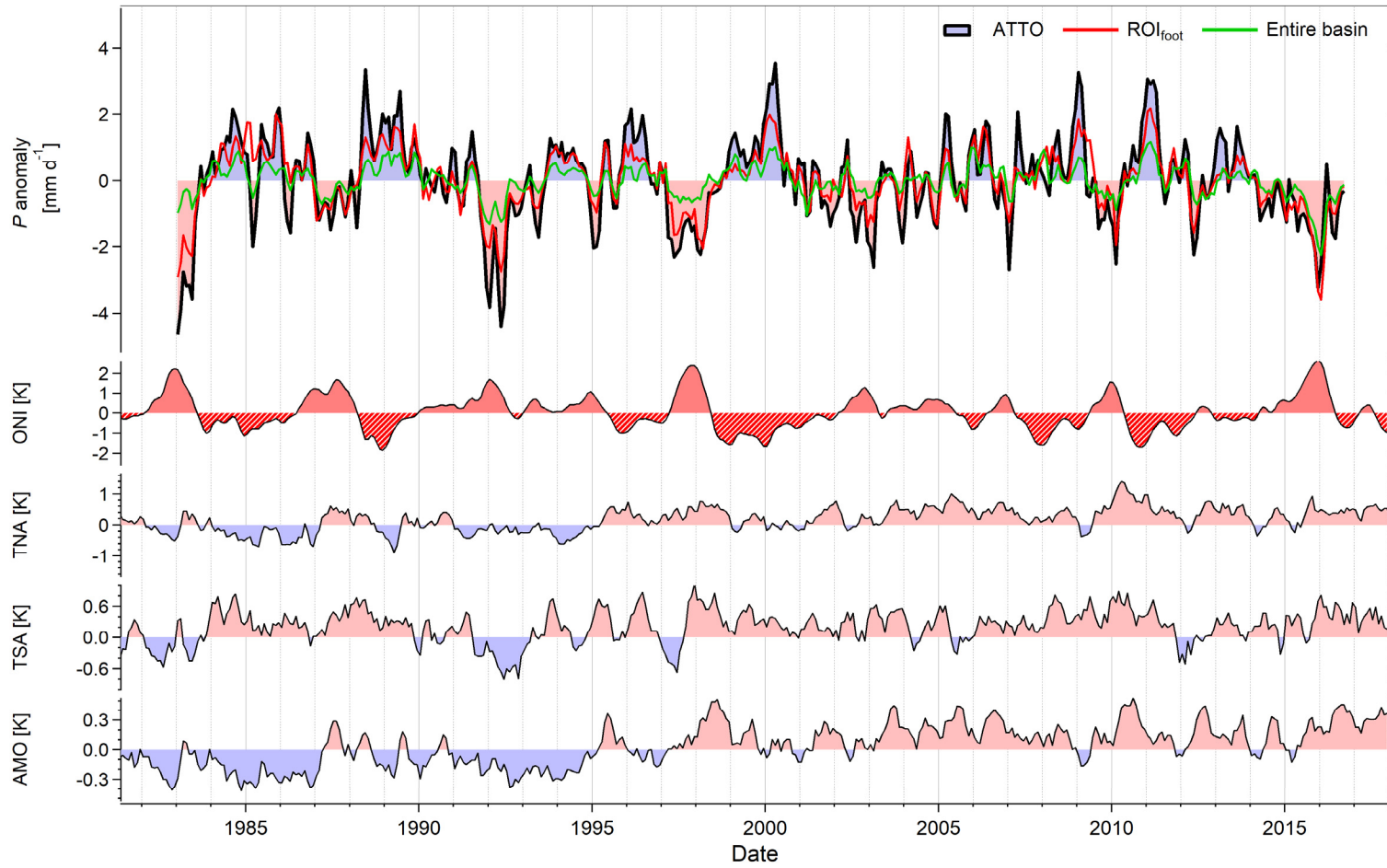
Figure S12. Anomalies in precipitation rate P for the ATTO region (see Fig. 4), the \text{ROI}_{\text{foot}} (continental part only, see Fig. 4 and 7), and the entire basin (see Amazon watershed region in Fig. 7). Pacific and Atlantic sea surface temperature indices are shown for comparison: Oceanic Niño index (ONI), representing Pacific SST variability and indicating El Niño vs. La Niña periods (i.e., El Niño influence is very strong for \text{ONI} > 2.0 , strong for 2.0 > \text{ONI} > 1.5 , medium for 1.5 > \text{ONI} > 1.0 , and weak for \text{ONI} > 1.0 ). La Niña influence is strong for -2.0 < \text{ONI} < -1.5 , medium for -1.5 < \text{ONI} < -1.0 , and weak for \text{ONI} > -1.0 ). Tropical Northern Atlantic (TNA) and tropical Southern Atlantic (TSA) indices, representing Atlantic SST variability. Atlantic Multidecadal Oscillation (AMO) index.
