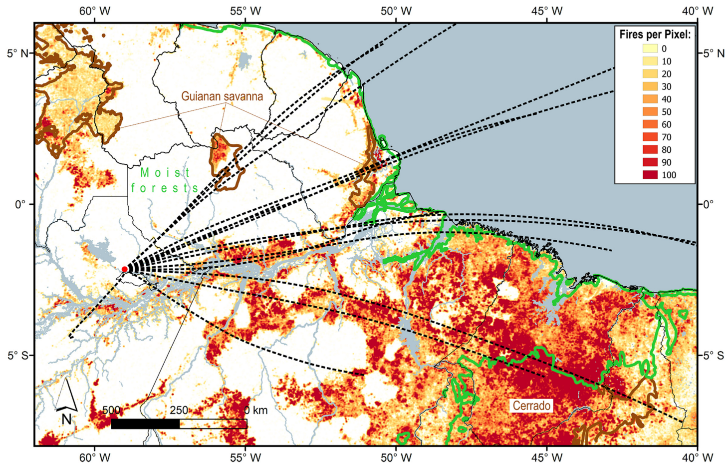
Figure S17. Map of the ATTO-relevant eastern Amazon Basin (ROI foot ) combining the backward trajectory (BT) data with two GIS data layer: (i) map of satellite detected fires within time period from 1998 to 2016 based on INPE data base and (ii) biome classification (see Fig. 9a). The BT data is represented as center lines of the 15 BT clusters (black dashed lines, see Fig. 4).
