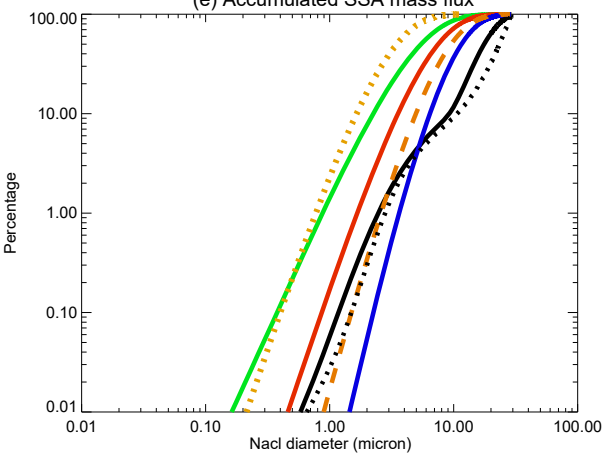
(e) Accumulated SSA mass flux
