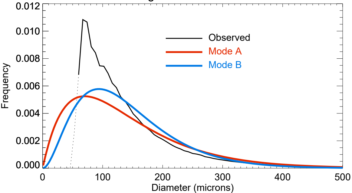
Blowing-snow size distribution
