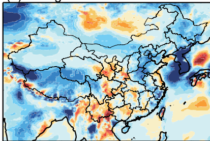
(a) Background PAN concentration
