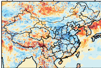
(b) Ozone dry deposition velocity
