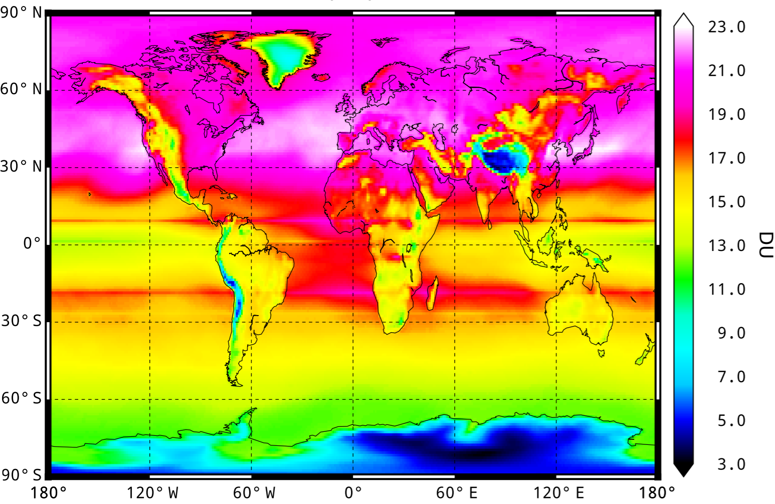
Mean FAT tropospheric column
