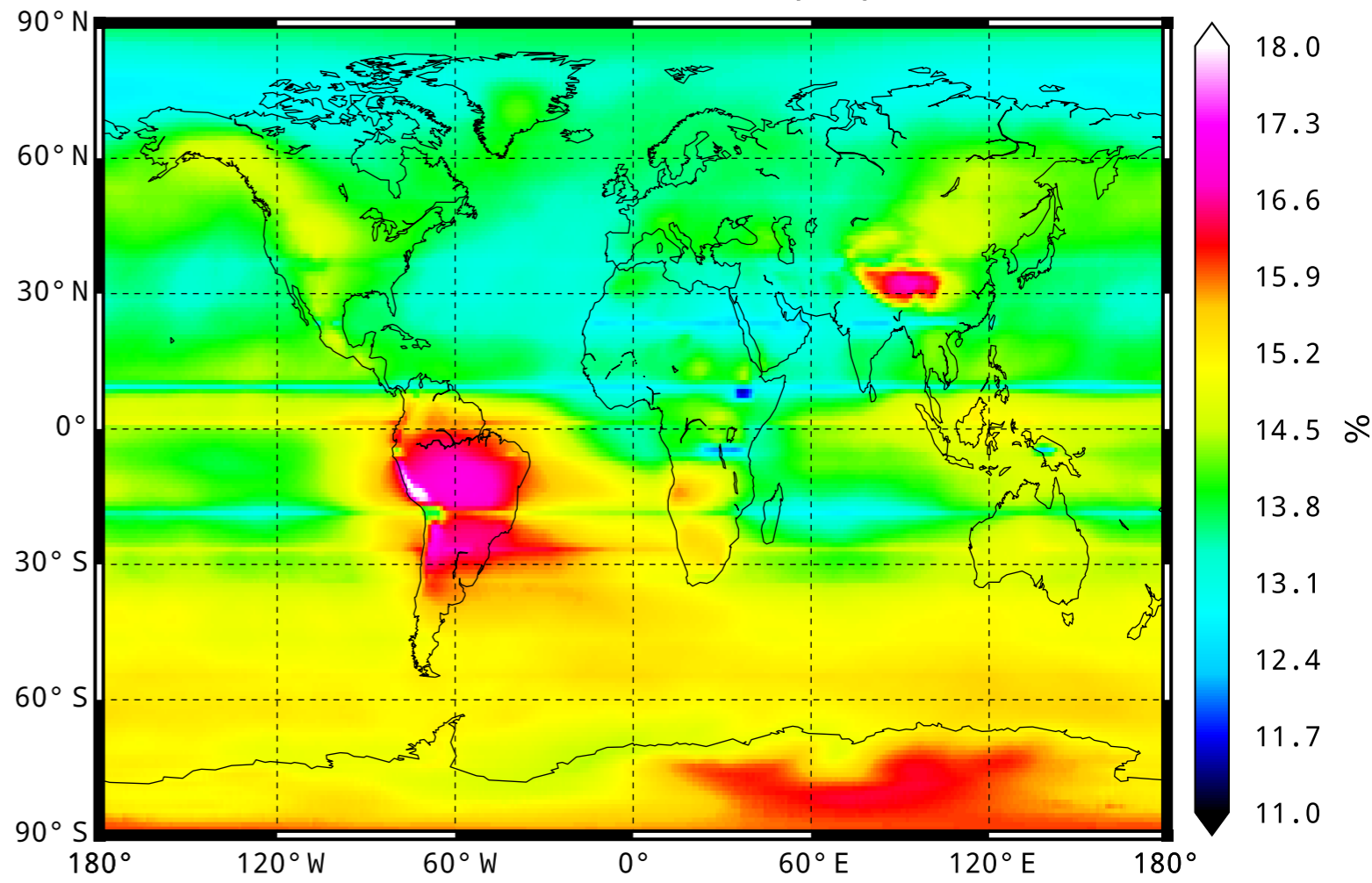
Relative error on the mean FAT tropospheric column
