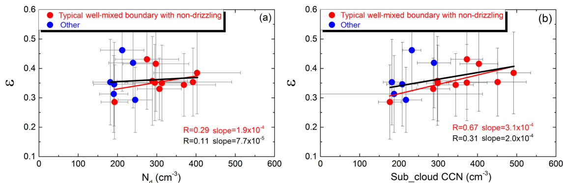
Figure 10. Relative dispersion ( \varepsilon ) as a function of (a) N_d and (b) sub-cloud CCN concentrations ( SS = 0.2\% ) for all flights. The error bars through these symbols indicate the standard deviation. Red symbols are the cases with typical well-mixed BL, and blue symbols are for other cases. Red (black) texts are the correlation coefficient and slope for typical well-mixed cases (all cases).
