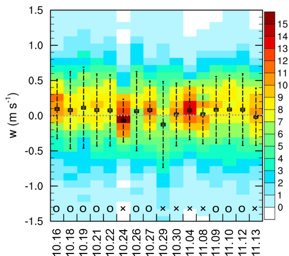
Figure 9. Probability distribution function (unit: %) of vertical velocity ( w ) for 16 non-drizzling flights. Black symbols are mean values of w , and error bars through these symbols indicate the standard deviation. Circles are the cases with typical well-mixed BL, and crosses represents the other cases.
