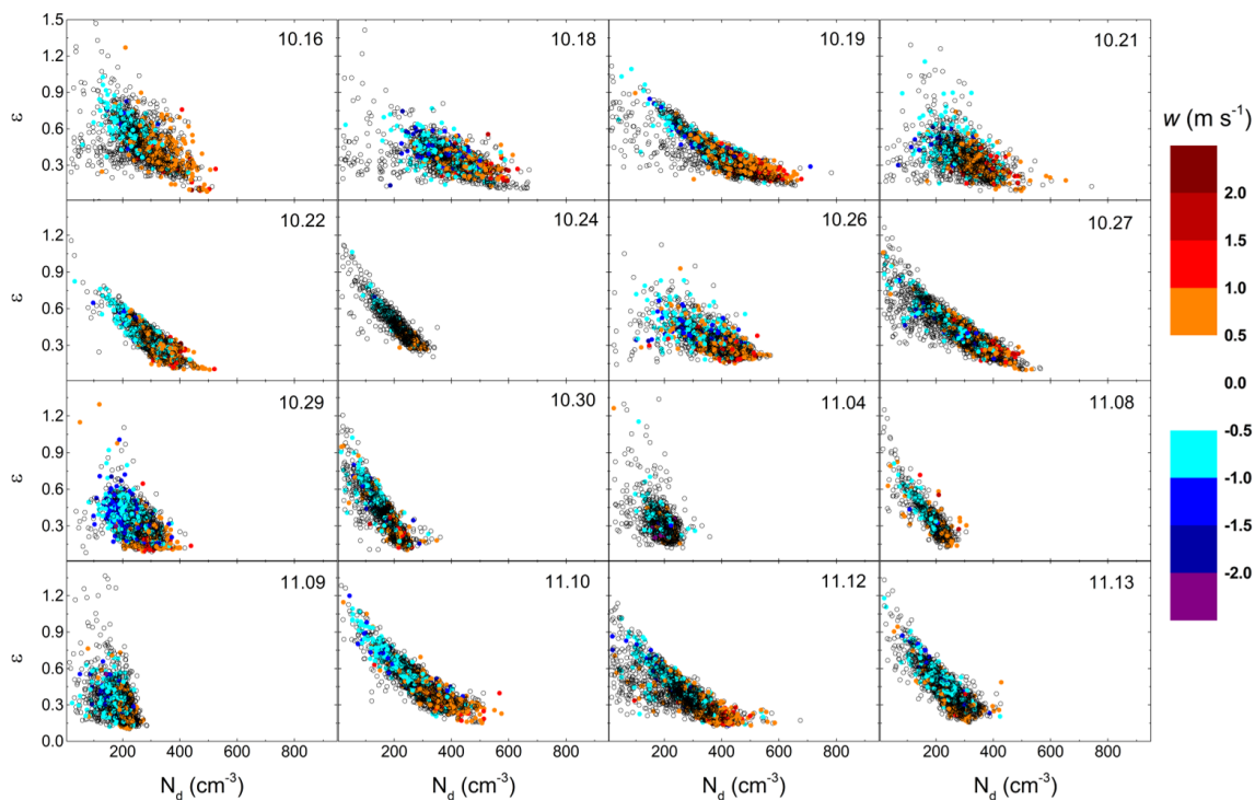
Figure 8. Relationships between relative dispersion ( \epsilon ) and N_d during all 16 non-drizzling flights, in which the color represents in-cloud vertical velocities ( \text{m s}^{-1} ).
