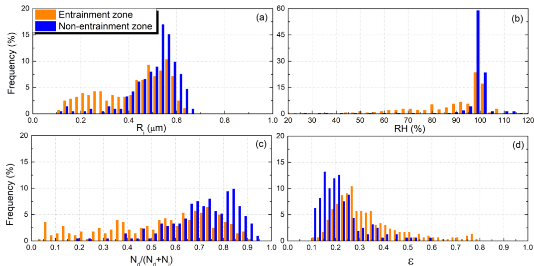
Figure 12. Probability density functions of (a) R_i ( \mu\text{m} ), (b) RH (%), (c) N_d/(N_d + N_i) , and (d) \varepsilon in the entrainment (orange) and non-entrainment zones (blue) during the flight on 18 October.
