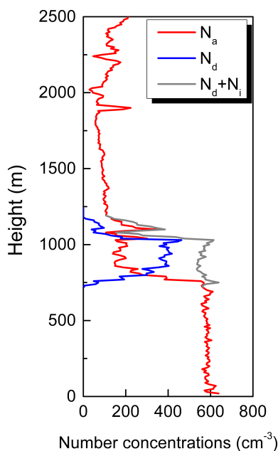
Figure 5. Vertical profiles of number concentrations of aerosols ( N_a ), cloud droplets ( N_d ), and total in-cloud particles ( N_d + N_i ) during the flight on 18 October.
