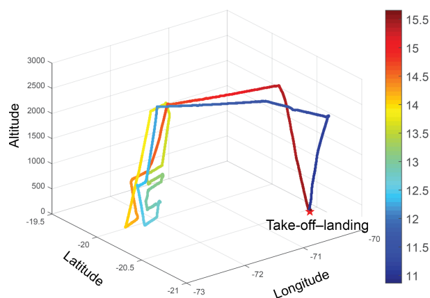
Figure 1. The flight track in 18 October; the colors represent flight time in hours (UTC).
