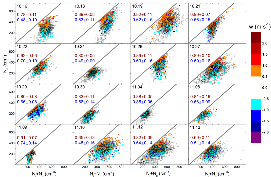
Figure 6. Relationships between N_d and N_i + N_d during all 16 non-drizzling flights. The color represents in-cloud vertical velocities ( \text{m s}^{-1} ), and gray line is 1 : 1 line. The mean and standard deviation of N_d/(N_d + N_i) for vertical velocity greater than 1 \text{ m s}^{-1} (red) and less than -1 \text{ m s}^{-1} (blue) are shown.
