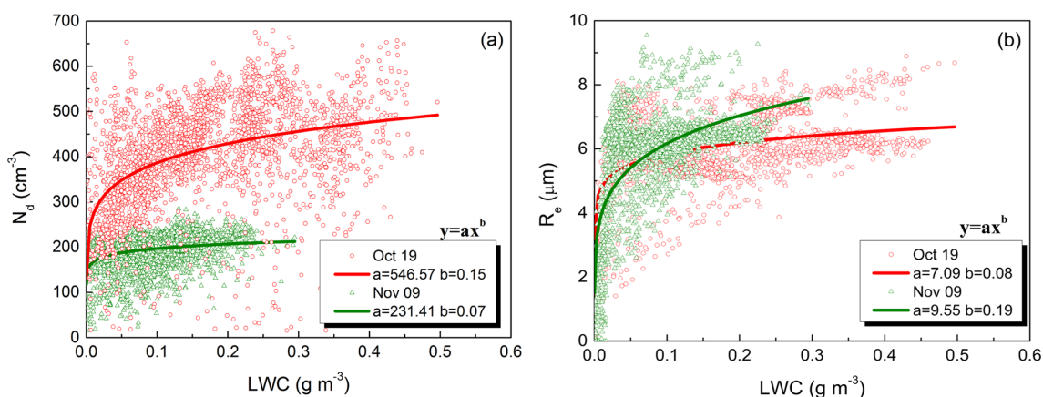
Figure 4. Correlations between (a) N_d ( \text{cm}^{-3} ), (b) R_e ( \mu\text{m} ), and LWC ( \text{g m}^{-3} ) for clean (green) and polluted (red) cases, respectively.
