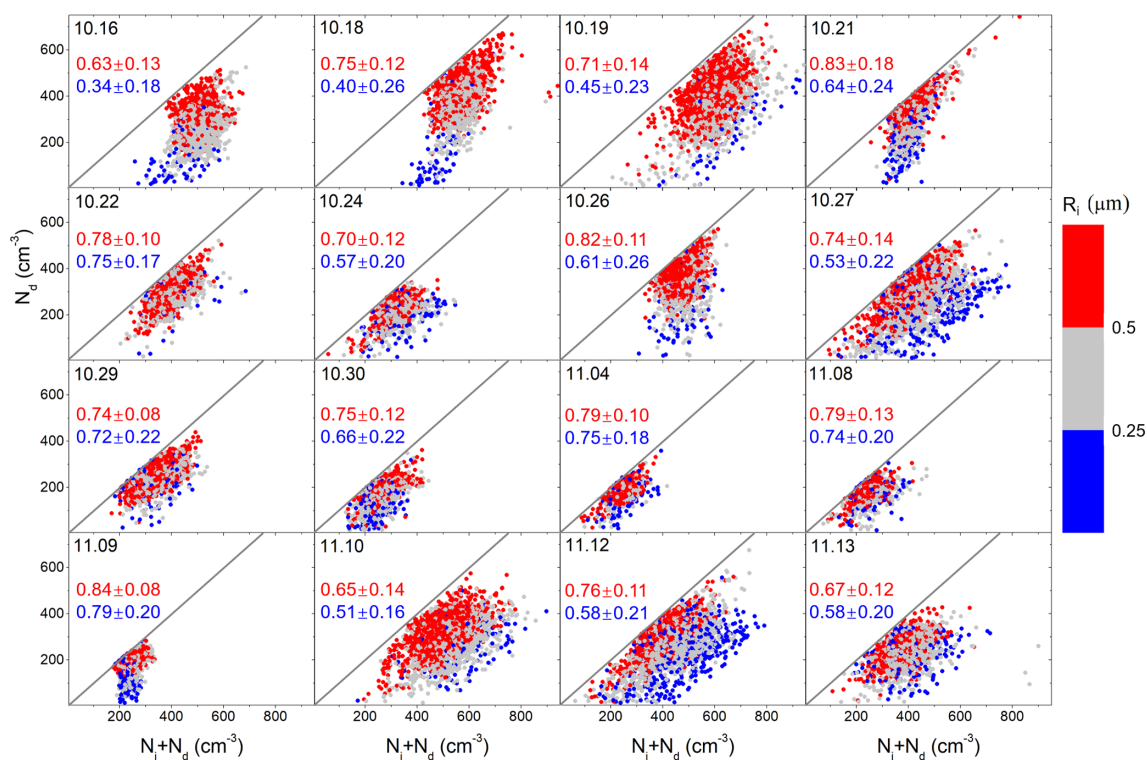
Figure 7. Same as Fig. 6, but the color represents the effective radius of interstitial aerosol ( R_i ; \mu\text{m} ). The mean and standard deviation of N_d/(N_d + N_i) for R_i greater than 0.5 \mu\text{m} (red) and less than 0.25 \mu\text{m} (blue) are shown.
