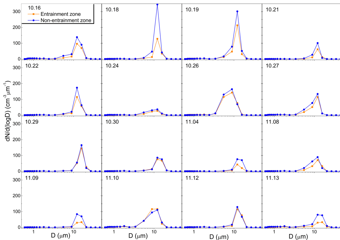
Figure 11. Number size distributions of cloud droplets in the entrainment (orange) and non-entrainment zones (blue) during all 16 non-drizzling flights.
