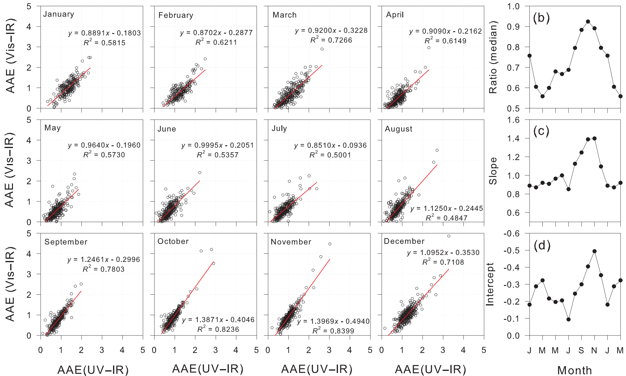
(a) Relation between AAE_{UV-IR} and AAE_{Vis-IR}
