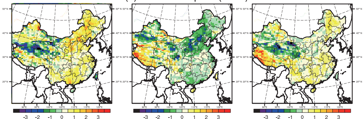
(e) 10 m wind speed ( \text{m s}^{-1} )
